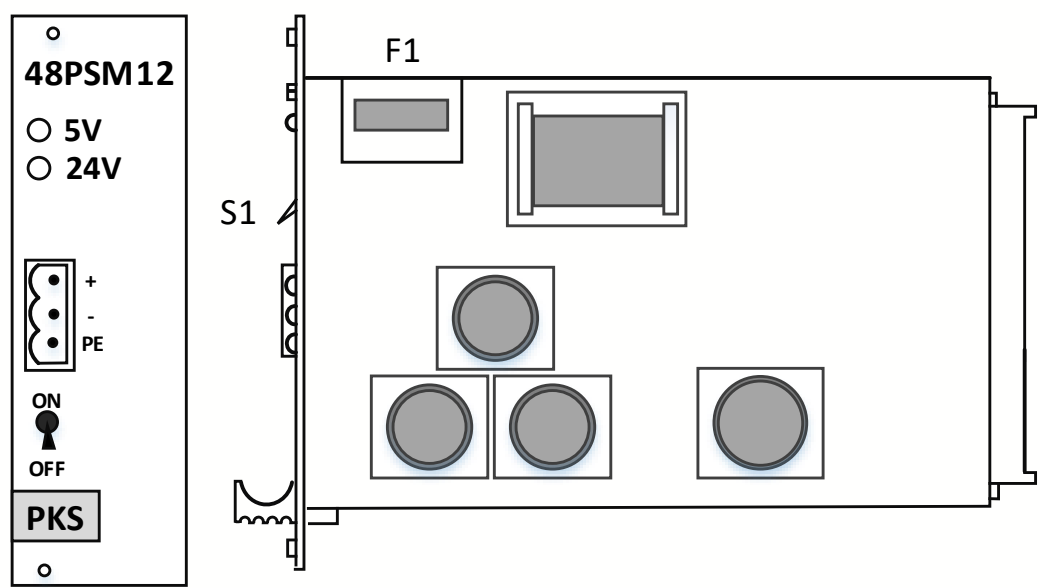
Fig.2: Board Layout and Fuse Position
